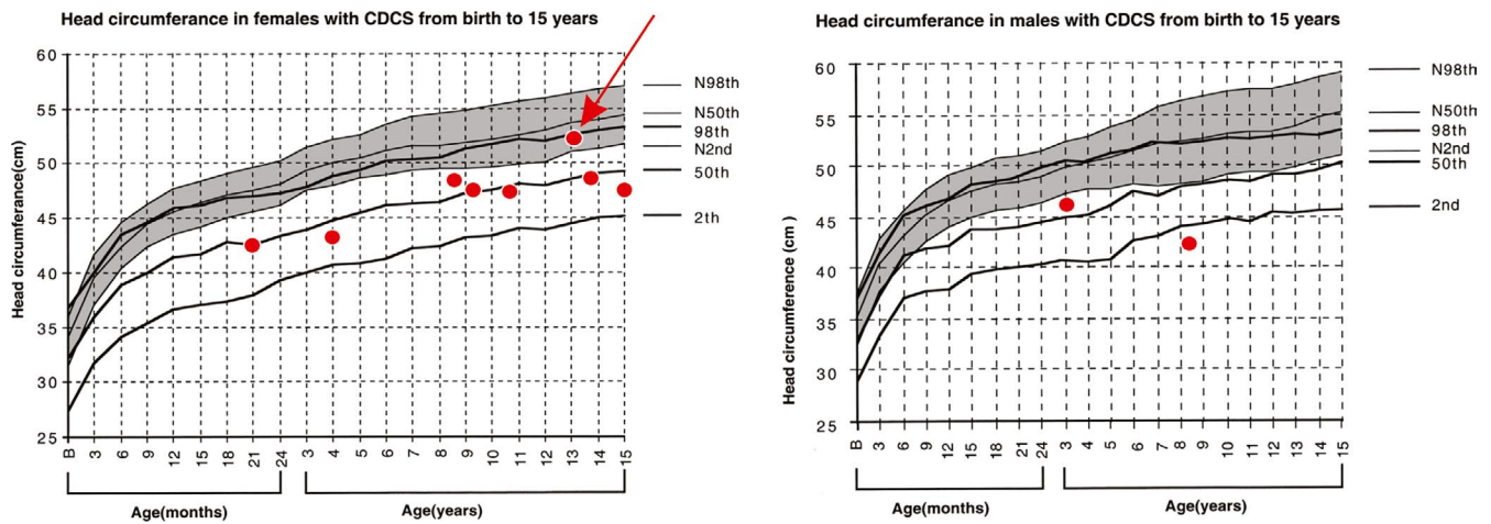
FIGURE 1 Head circumference in females and males with CdCS from birth to 15 years. Normal growth curves (N) are represented by the grey area and CdCS specific curves are indicated by the thick black lines. The results found in our 10 patients (red circles) showed that only one patient (patient 14) appears to have no microcephaly (red arrow) with measurements between 2nd <math>p</math> <math>< 50</math>th for normal growth curves and 98th for CdCS' growth curves. Adapted from Marinescu et al. (2000). CdCS, cri du chat syndrome
